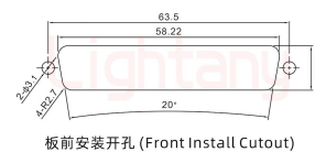
板前安装开孔 (Front Install Cutout)
